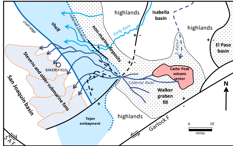
Caliente River Deposition System of Saleeby et al. (2016)
