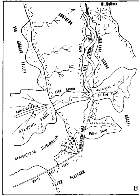
Miocene Stream Capture Model of MacPherson (1978)
